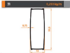
Ahşap Jaluzi Perde Etek Profil Venetian Blind Bottomrail Profile
